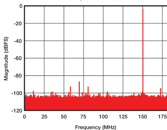
1 -Tone Spectrum, 150 MHz
