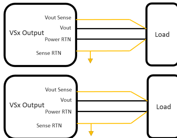
Figure 3: M4465 Sense line connection
