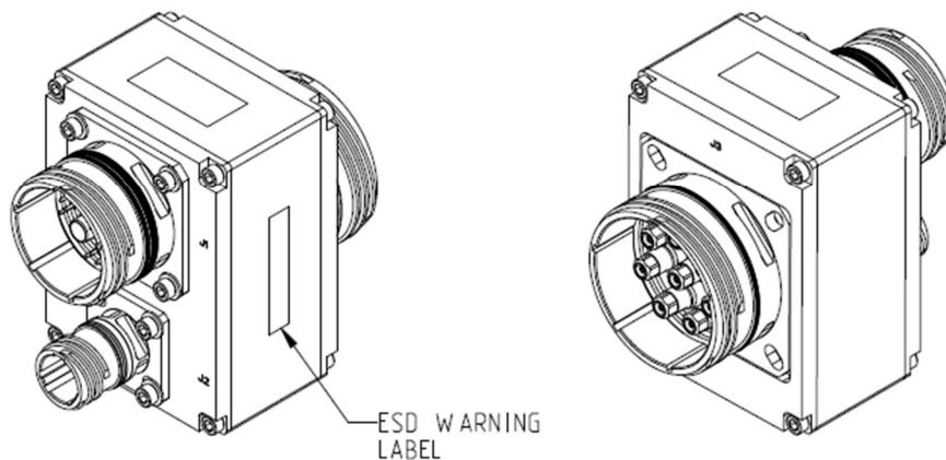
DETAIL B J3 CONNECTOR SCALE 3.000
