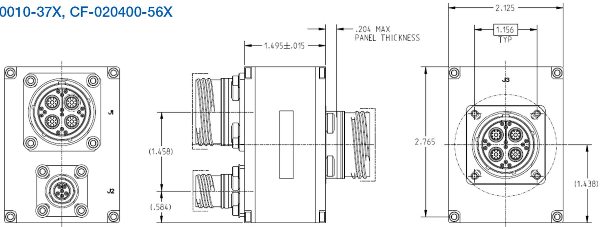
CF-020010-37X Pinout
