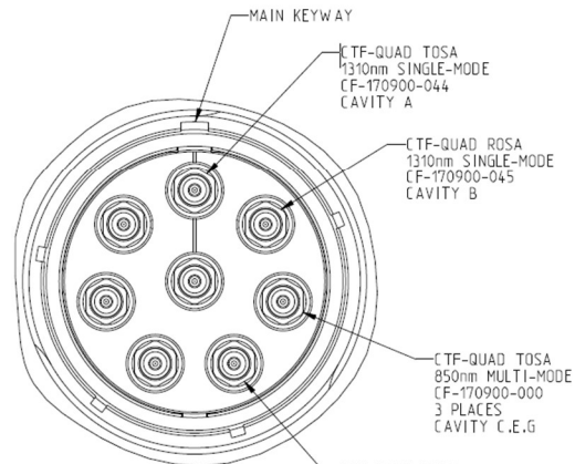
DETAIL B J3 CONNECTOR SCALE 3.000
