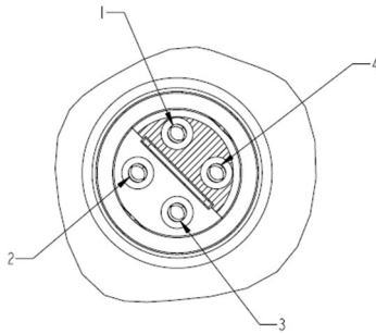
DETAIL A J2 CONNECTOR FRONT VIEW SPLIT-PAIR QUAD
