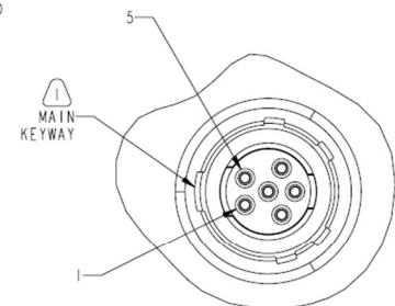
DETAIL C (INSERT ARRANGEMENT L-21809-6) SCALE 4.000
