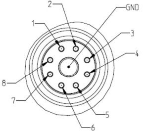
DETAIL A OCTONET PIN POSITION SCALE 8.000
