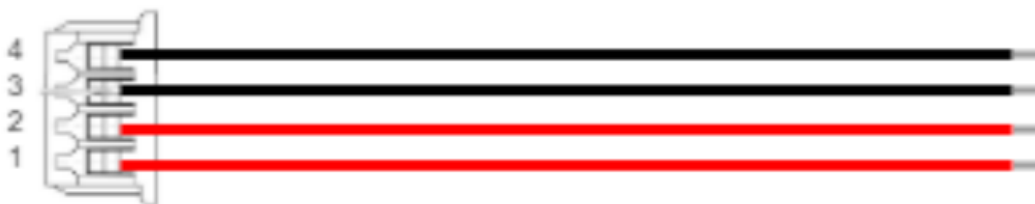
Voltage input cable pinout (red = V+, black = GND)
