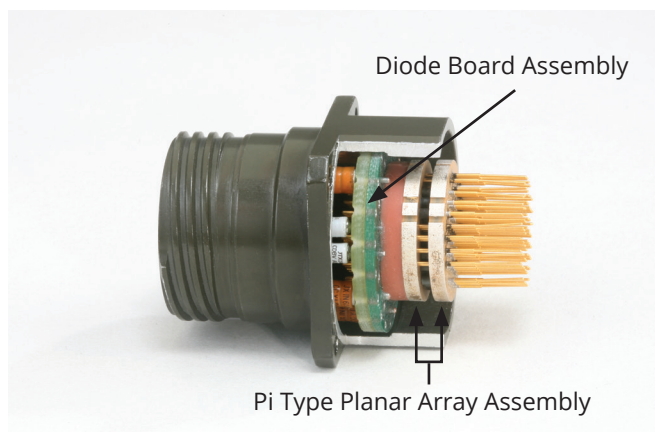
Dual Transient and Filter Connector Cross Section
