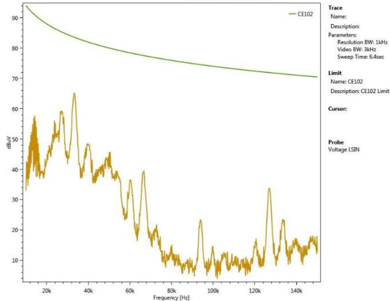
CE102 MIL-STD-461F Conducted Emission, 10 kHz -150 kHz
