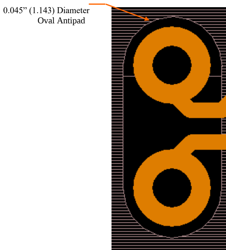
Figure 9: Antipad Clearance – Daughtercard Connector
