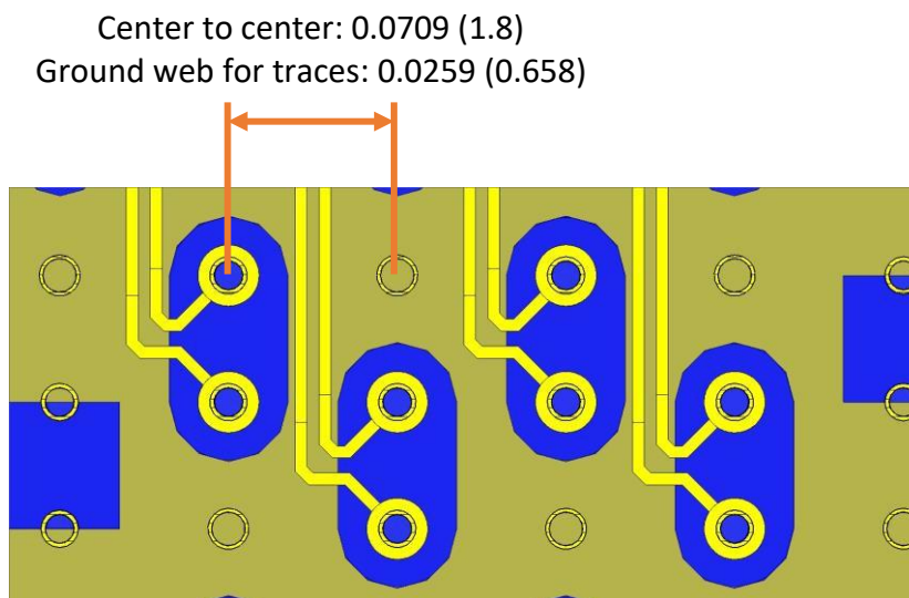
Figure 10: Example Daughtercard High Speed Differential Routing
