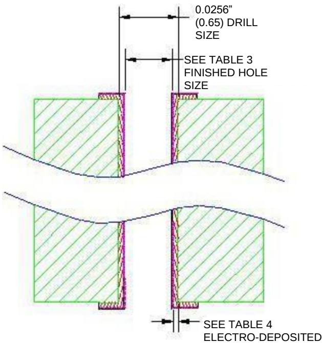
Figure 2: BP Tail (0.0256") Drill and Finished Hole Size
