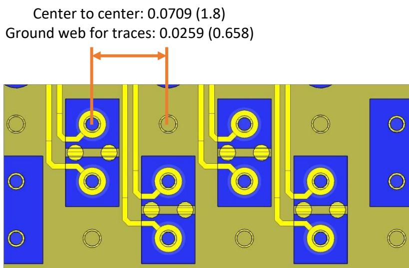
Figure 18: Example Backplane Typical High Speed Differential Routing Ground Plane
