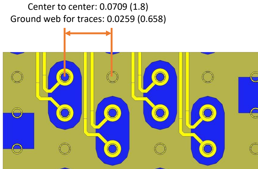
Figure 14: Example Backplane Typical High Speed Differential Routing Ground Plane
