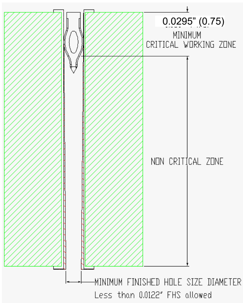
Figure 7: Femto Tail (0.0157") Compliant Pin Critical Zone
