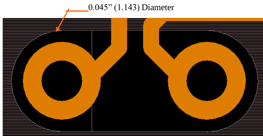
Figure 8: Antipad Clearance – Backplane Connector
