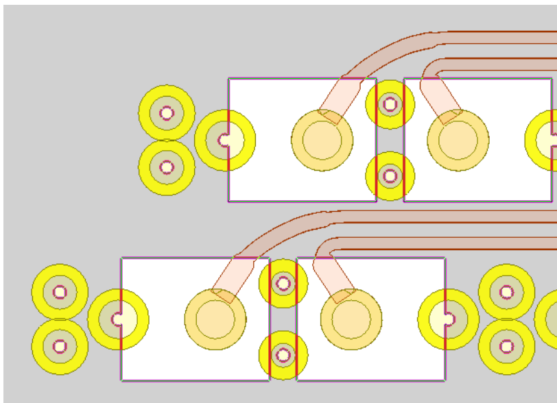
Figure 12: Example Daughtercard Typical High Speed Differential Antipad Design
