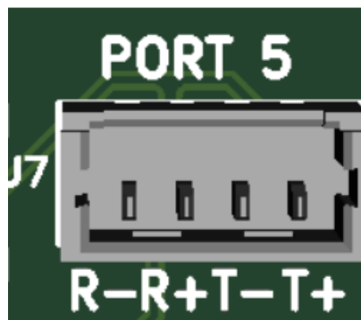
Ethernet port pinout for the Molex PicoBlade variant
