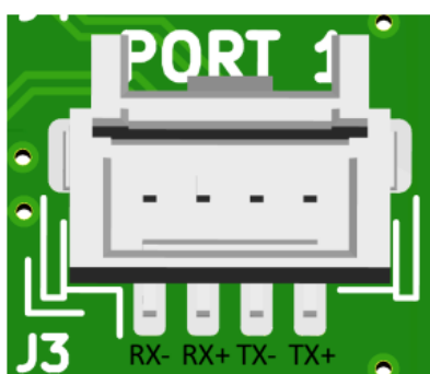
Ethernet port pinout for the Molex PicoClasp variant
