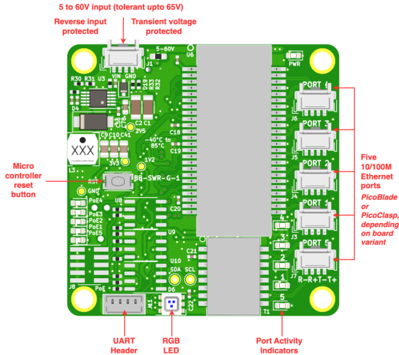
Board Map (back)
