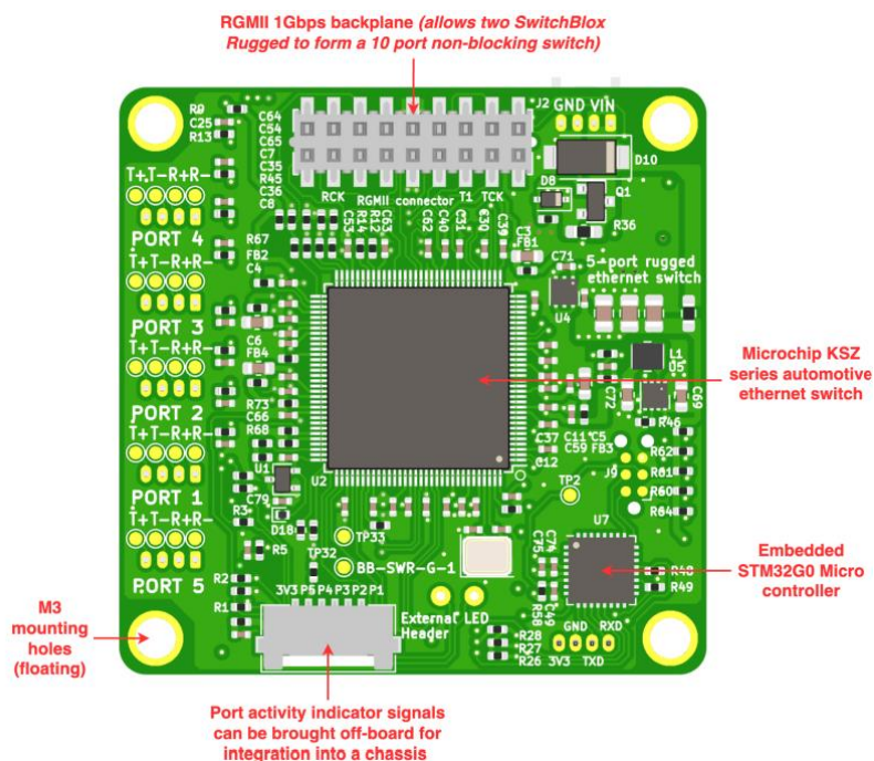
Board Map (back)
